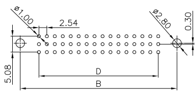
RECOMMEND PCB LAYOUT(FOR FEMALE) TOLERANCE=±0.05mm
